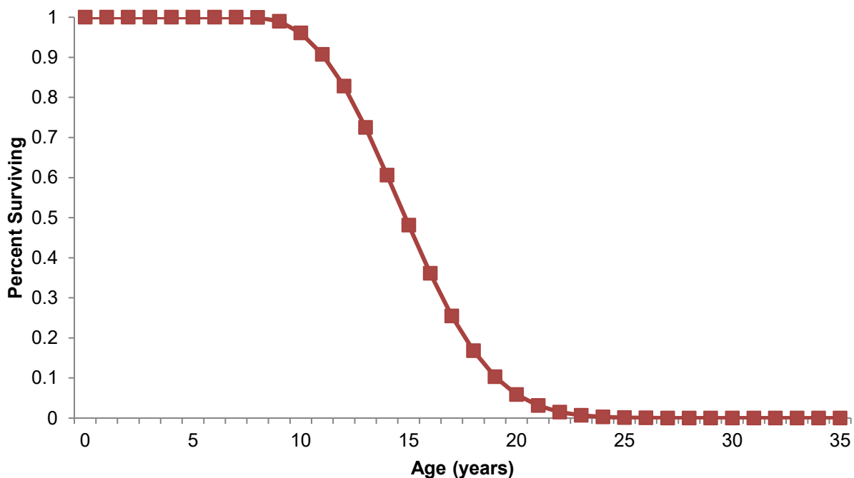
Figure 18.1-1: [Premium Motors] Survival Function 812
