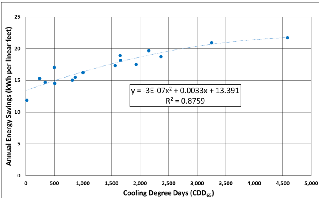
Figure 16.9-1: [Door Gaskets] Comparison of Projected Annual Energy Savings to Cooling Degree Days for All 16 California Climate Zones for Reach-In Display Cases (Coolers)
