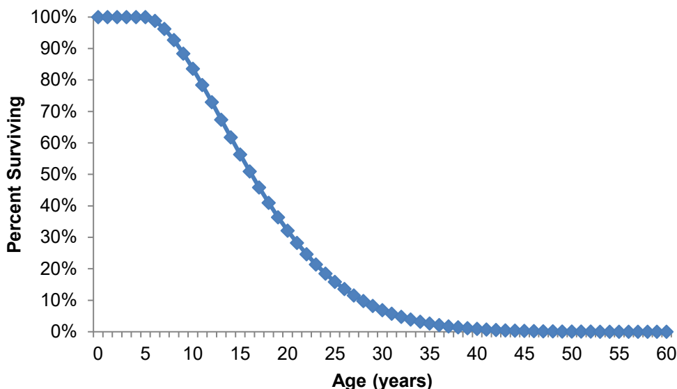
Figure 8.3-1: [Refrigerators] Survival Function 383
